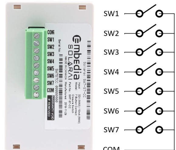
Example: label and contact configuration for SW7-S7-CC
